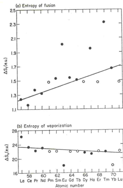
FIG. 30. (a) Entropy of fusion of the rare-earth metals. (b) Entropy of vaporization of the rare-earth metals. Open points are estimated data.
